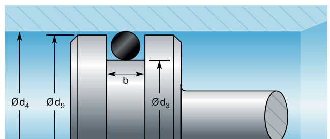
Fig. 3.13 Piston seal – radial compression
