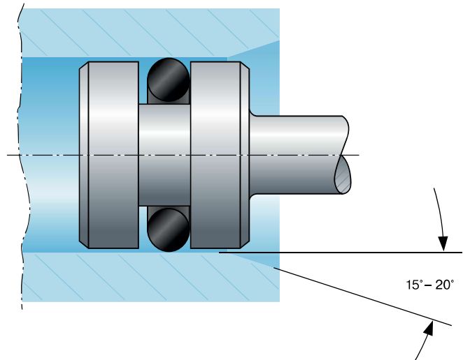
Fig. 2.22 Assembly example of piston
