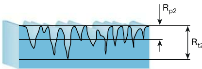
Surfaces produced by normal machining
