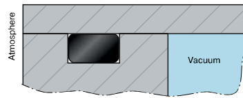
Fig. 7.5 Vacuum O-Ring gland
