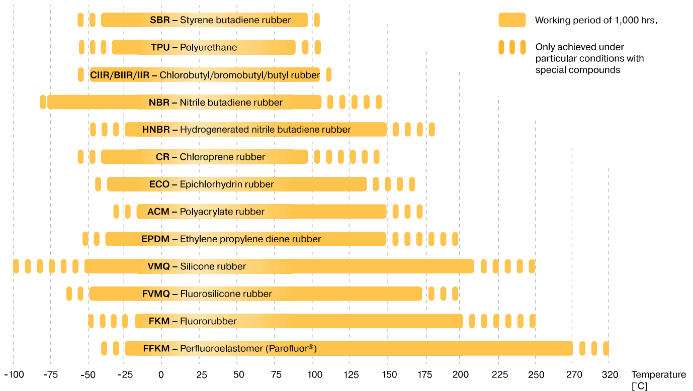
Fig. 7.2 High-temperature limits for various elastomeric materials
