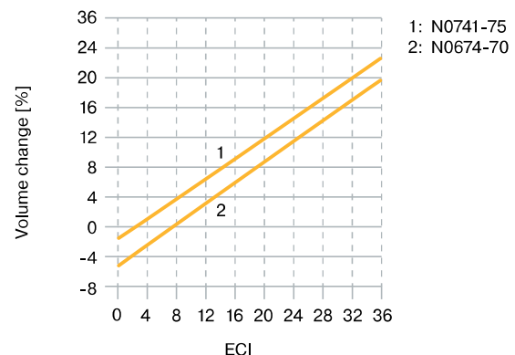
Fig. 8.8 Swelling characteristics of Parker compounds
