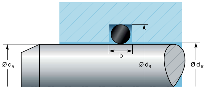
Fig. 3.2 Rod seal – radial compression
