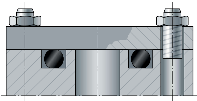
Fig. 2.3 Face seal: O-Ring deformed axially
