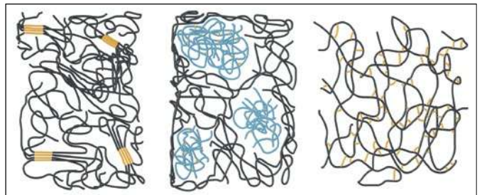
Block polymer (left), polymer blend (centre) Thermoplastic elastomers (left and centre), duroplastics – close-meshed crosslinking (right)
