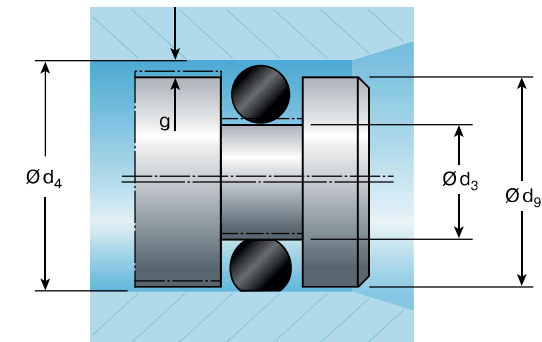
Fig. 8.35 With maximum radial play
