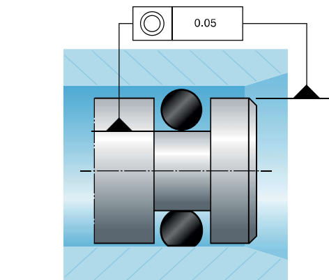
Fig. 8.36 With maximum eccentricity and non-concentric piston and groove diameters
