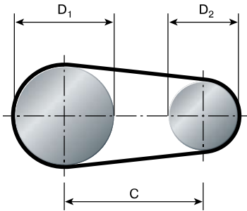
Fig. 2.19 Open design
