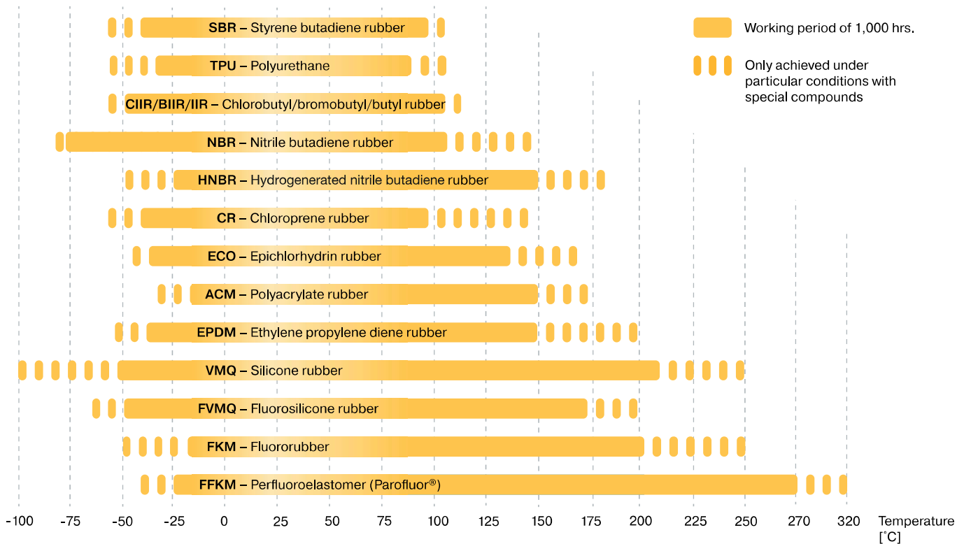
Fig. 6.4 High-temperature limits for various elastomeric materials
