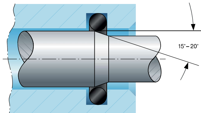
Fig. 2.23 Assembly example of rod
