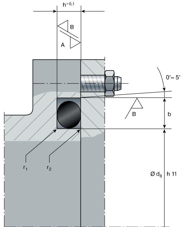
Fig. 2.9 Pressure from outside
