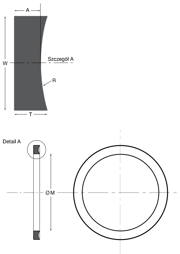
Fig. 4.11 Parbak® back-up ring
