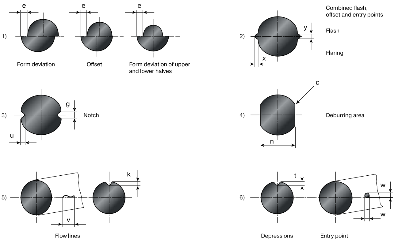
Fig. 9.1 Mould and surface finish defects
