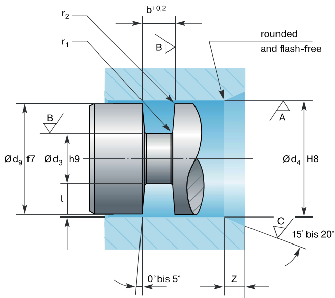
Fig. 2.5 Gland in inside element
