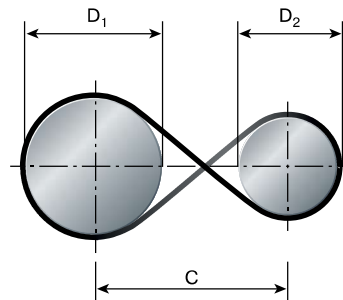
Fig. 2.20 Crossed design
