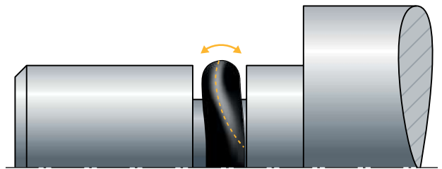
Fig. 2.28 O-Ring fitted rolled
