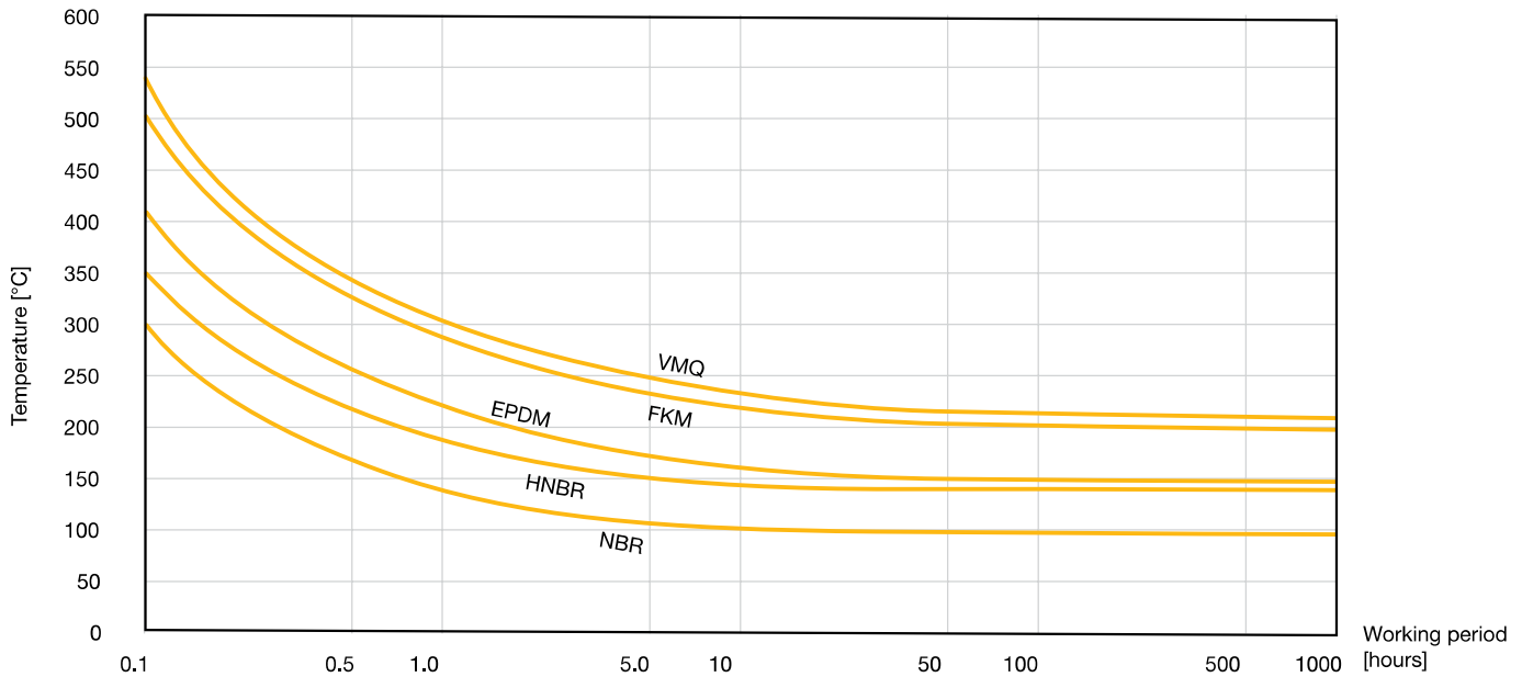
Fig. 7.1 High temperature limitations for various elastomeric materials
