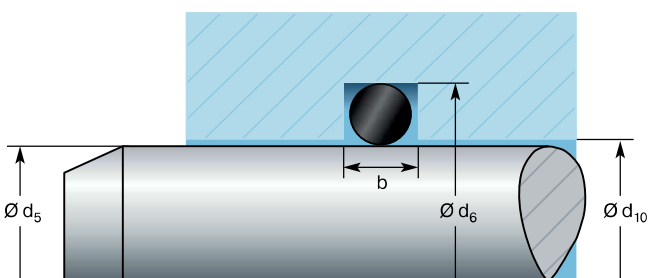
Fig. 3.14 Rod seal – radial compression
