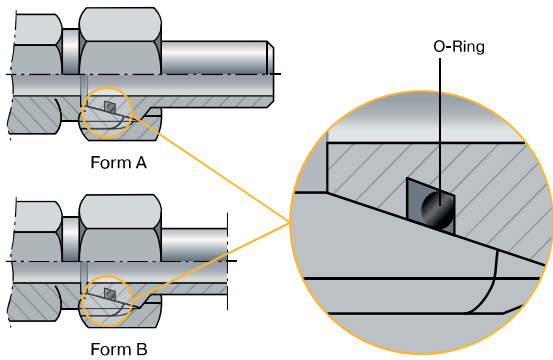
Fig. 4.4 Assembly
