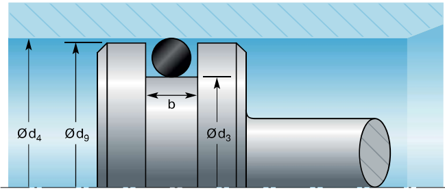
Fig. 3.1 Piston seal – radial compression
