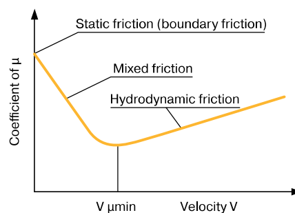
Fig. 8.18 Stribeck curve
