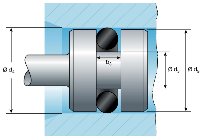
Fig. 3.15 Floating design – no deformation
