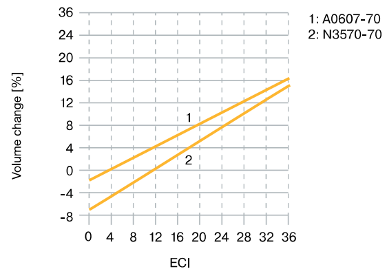
Fig. 8.7 Swelling characteristics of Parker compounds
