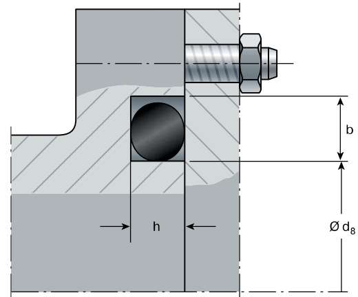
Fig. 3.4 Flange seal – axial deformation
