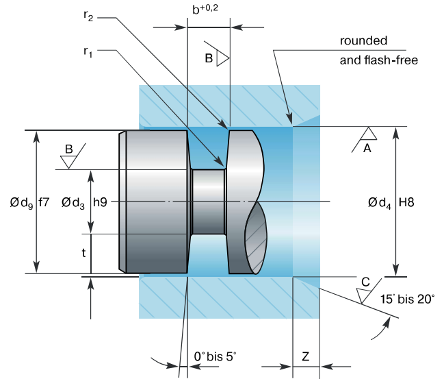
Fig. 2.15 Piston seal – hydraulic and pneumatic
